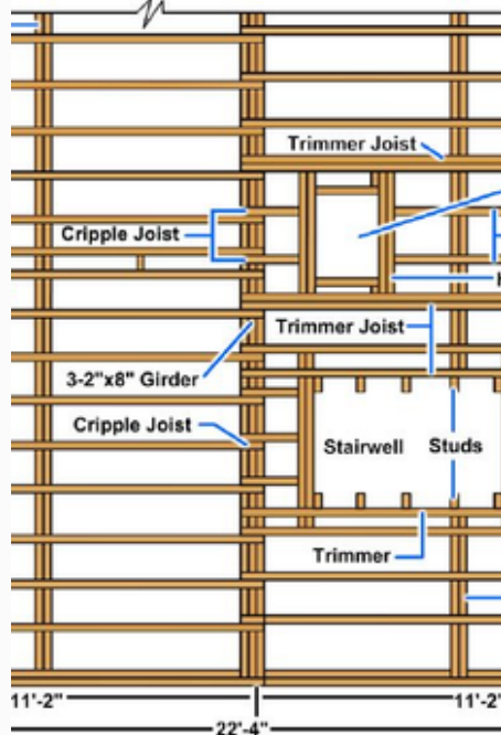
Figure 7-34 — Floor framing plan.
